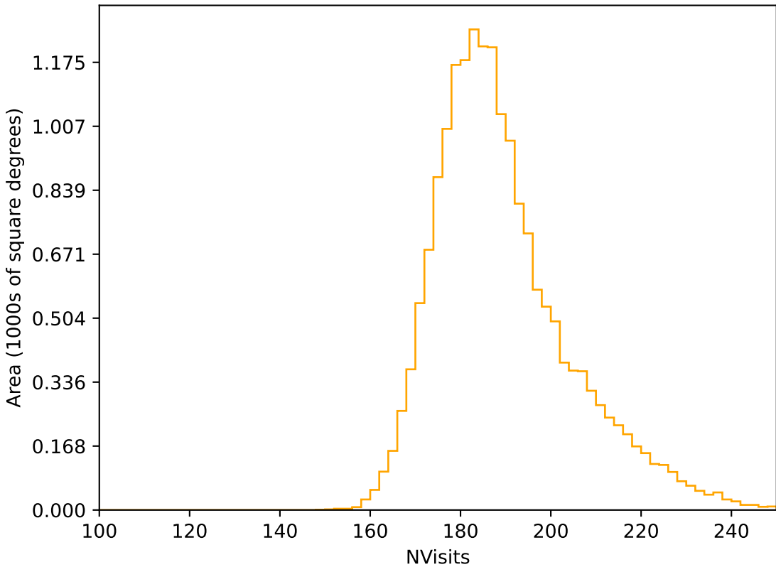
too_elab_r8_d2_gz_v3.4_10yrs WFD r band: NVisits
