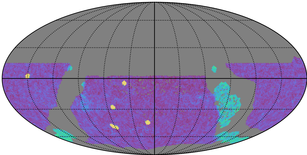
too_elab_r8_d2_gz_v3.4_10yrs WFD g band: NVisits
