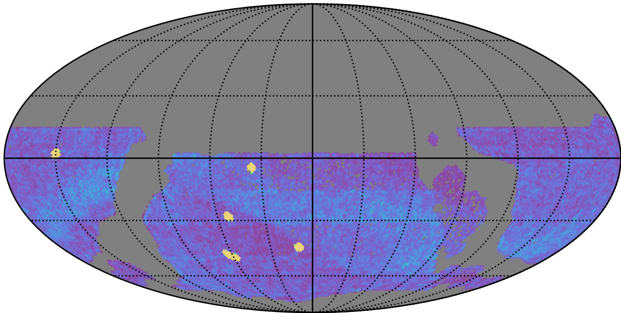
too_elab_r8_d2_gz_v3.4_10yrs WFD all bands: NVisits
