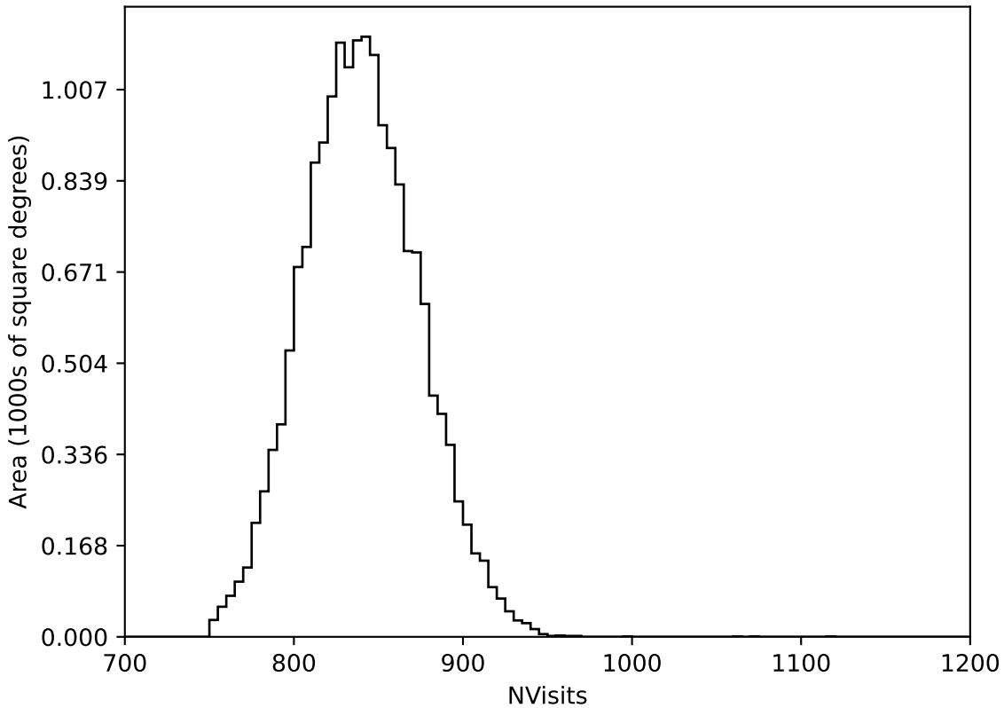
too_elab_r8_d2_gz_v3.4_10yrs WFD all bands: NVisits
