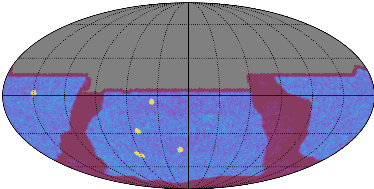
too_elab_r8_d2_gz_v3.4_10yrs All sky y band: NVisits
