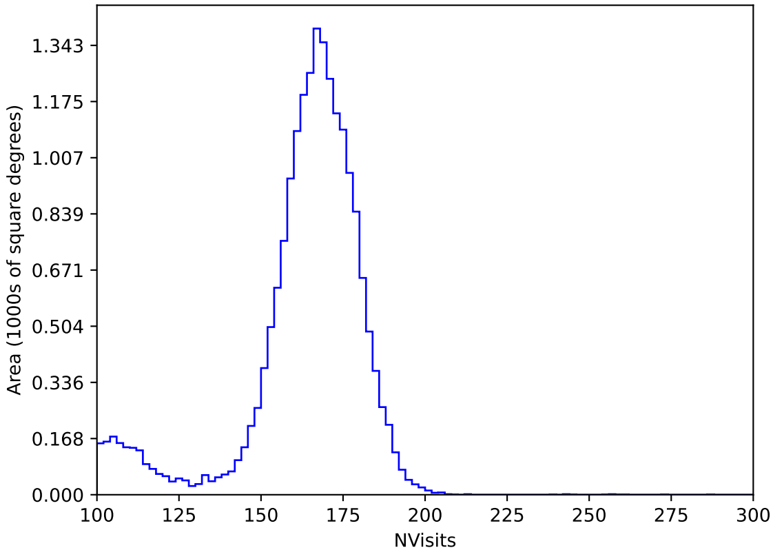
too_elab_r8_d2_gz_v3.4_10yrs All sky y band: NVisits
