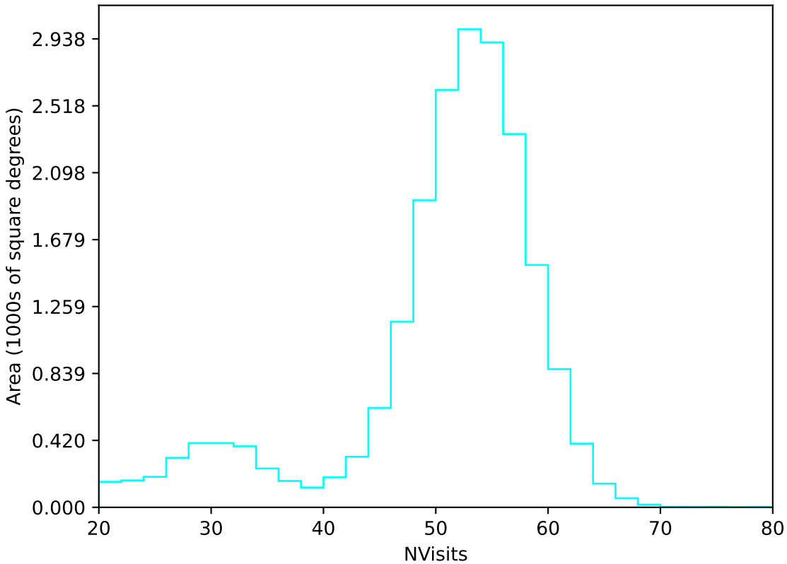
too_elab_r8_d2_gz_v3.4_10yrs All sky u band: NVisits
