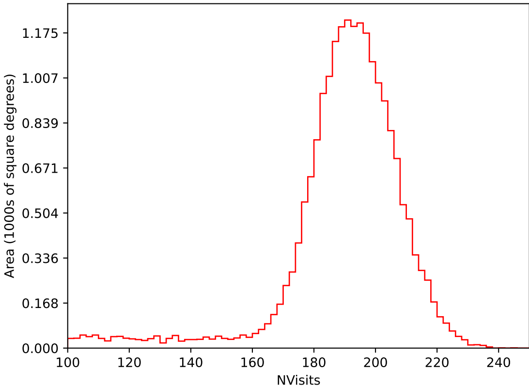
too_elab_r8_d2_gz_v3.4_10yrs All sky i band: NVisits
