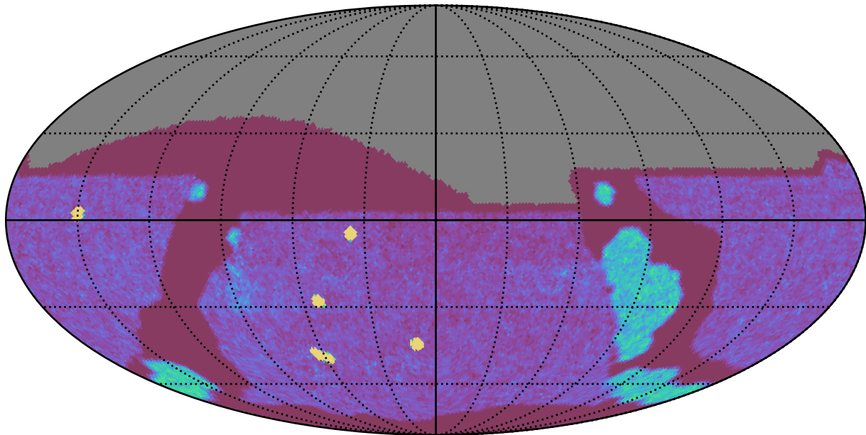
too_elab_r8_d2_gz_v3.4_10yrs All sky g band: NVisits
