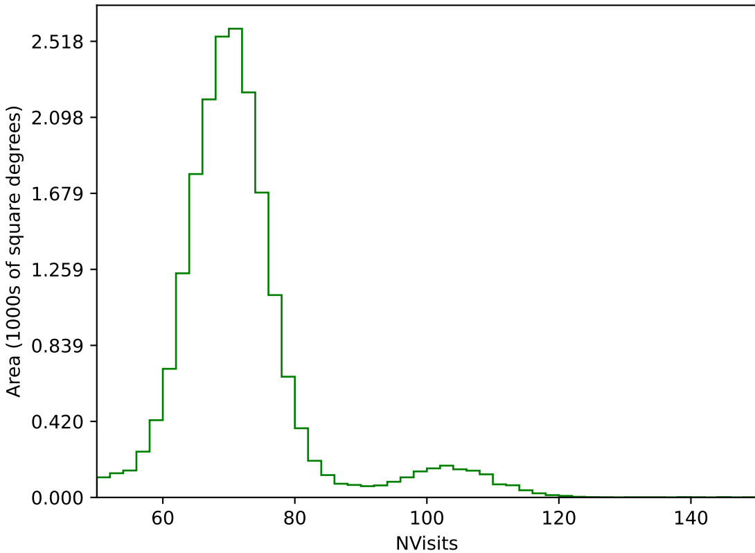
too_elab_r8_d2_gz_v3.4_10yrs All sky g band: NVisits
