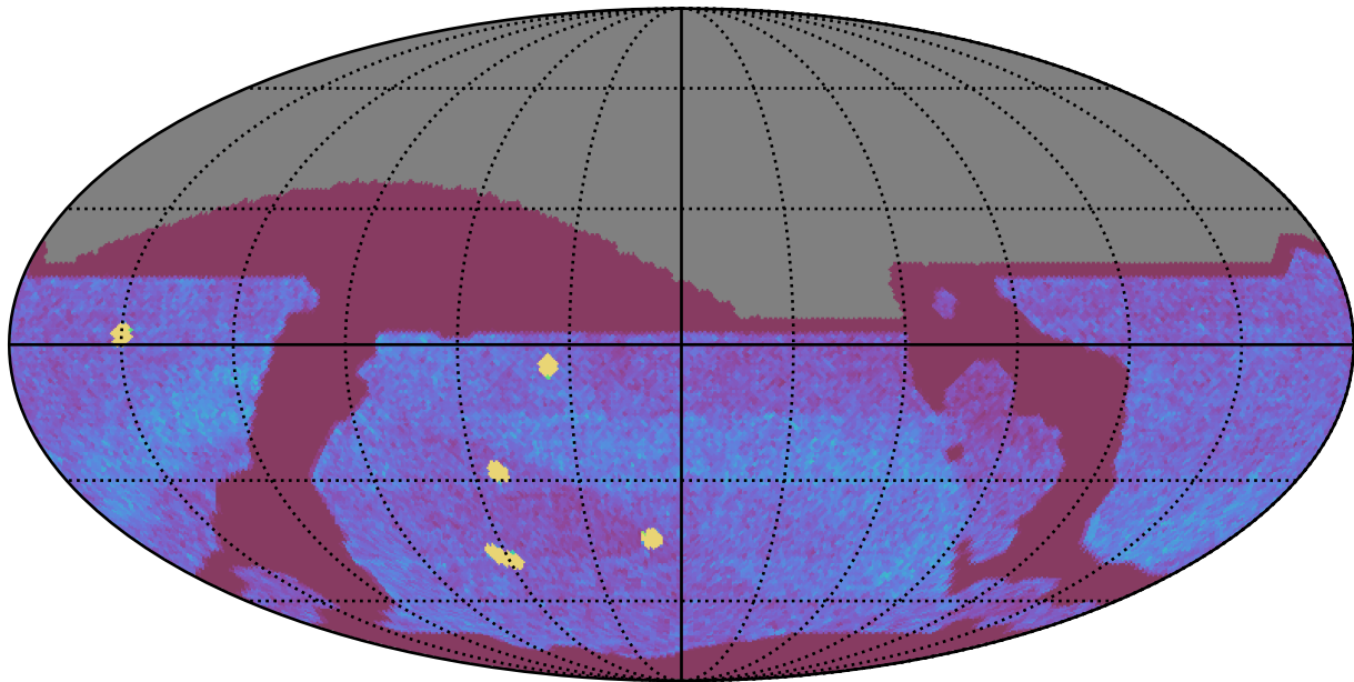
too_elab_r8_d2_gz_v3.4_10yrs All sky all bands: NVisits
