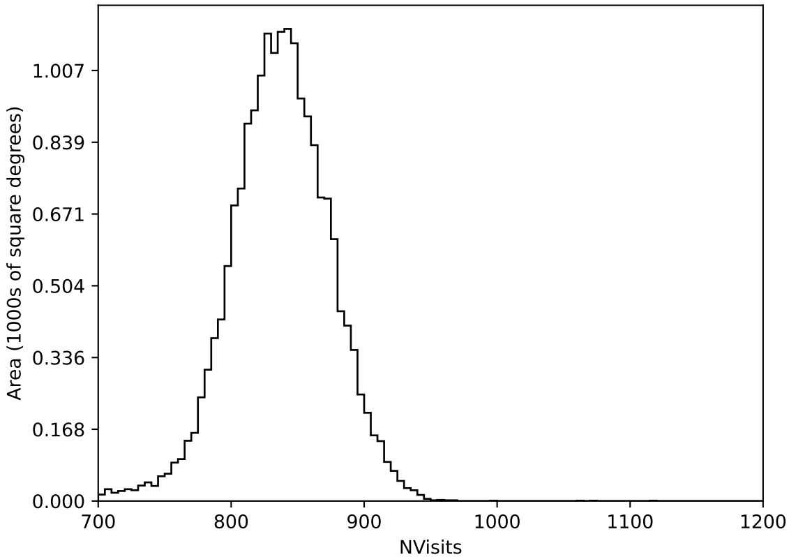
too_elab_r8_d2_gz_v3.4_10yrs All sky all bands: NVisits
