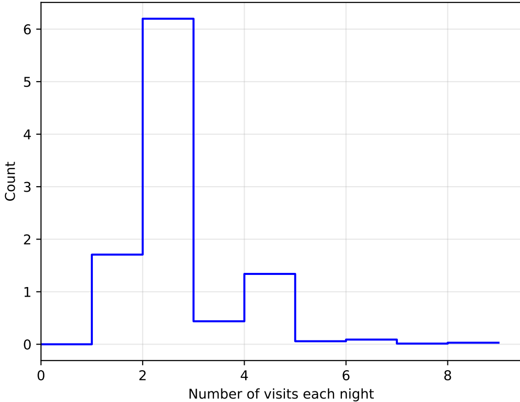
too_elab_r8_d2_gz_v3.4_10yrs All sky: NVisitsPerNight
