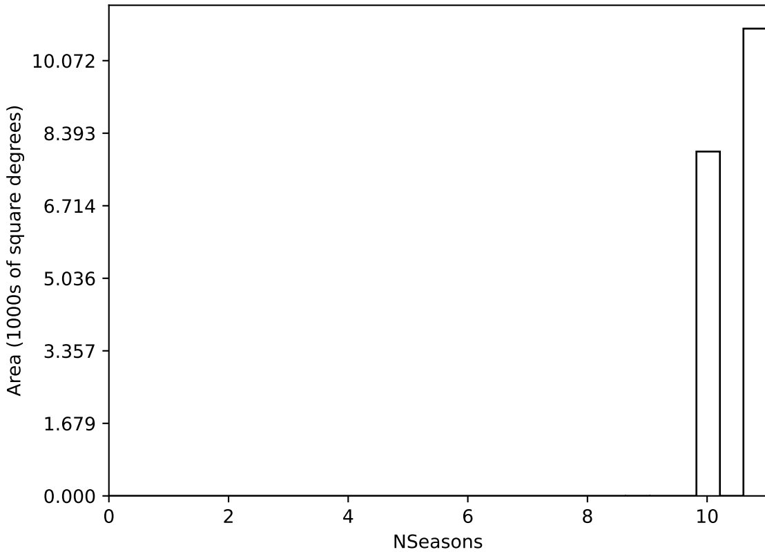
too_elab_r8_d2_gz_v3.4_10yrs WFD all bands: NSeasons
