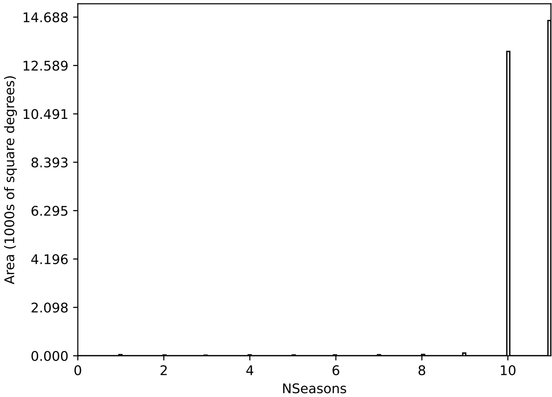
too_elab_r8_d2_gz_v3.4_10yrs All sky all bands: NSeasons
