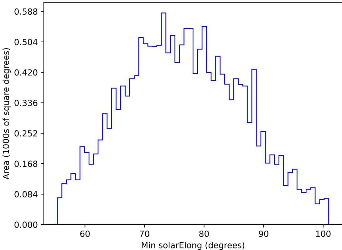
too_elab_r8_d2_gz_v3.4_10yrs WFD u band: Min solarElong
