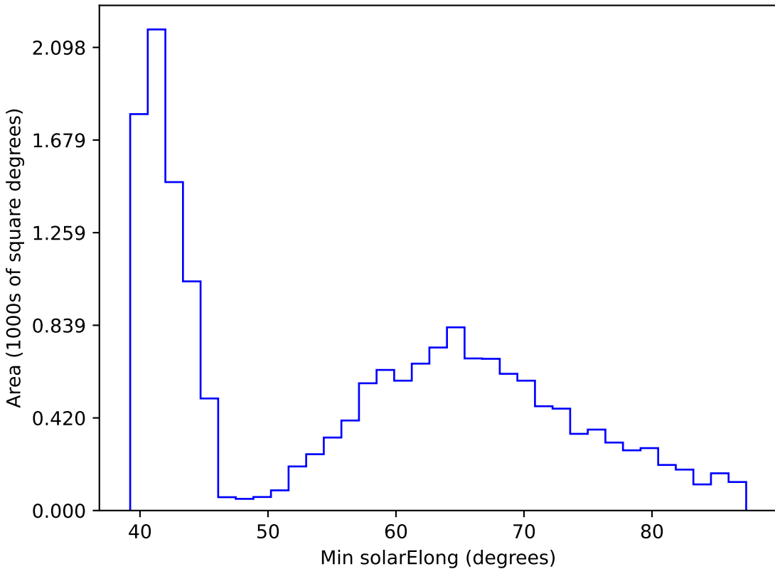
too_elab_r8_d2_gz_v3.4_10yrs WFD r band: Min solarElong
