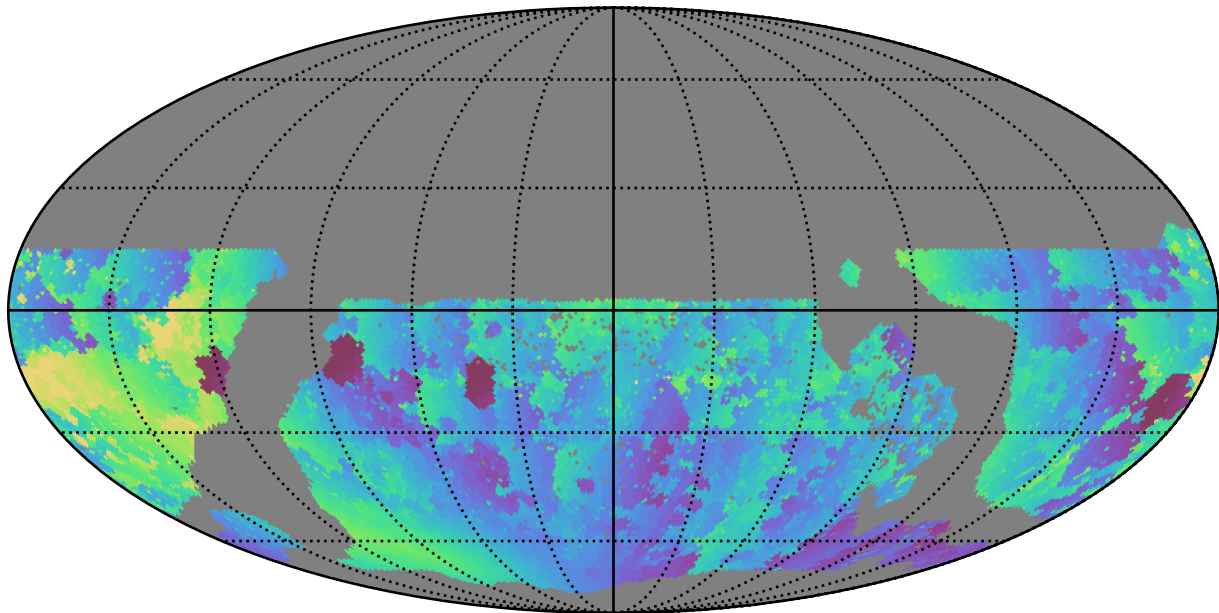
too_elab_r8_d2_gz_v3.4_10yrs WFD g band: Min solarElong
