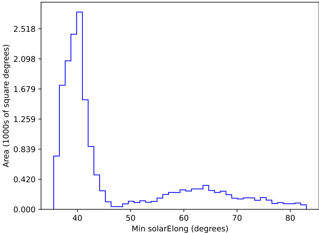
too_elab_r8_d2_gz_v3.4_10yrs WFD all bands: Min solarElong
