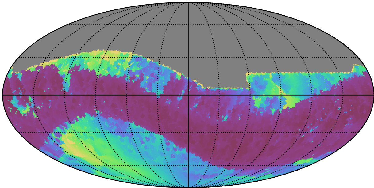
too_elab_r8_d2_gz_v3.4_10yrs All sky z band: Min solarElong
