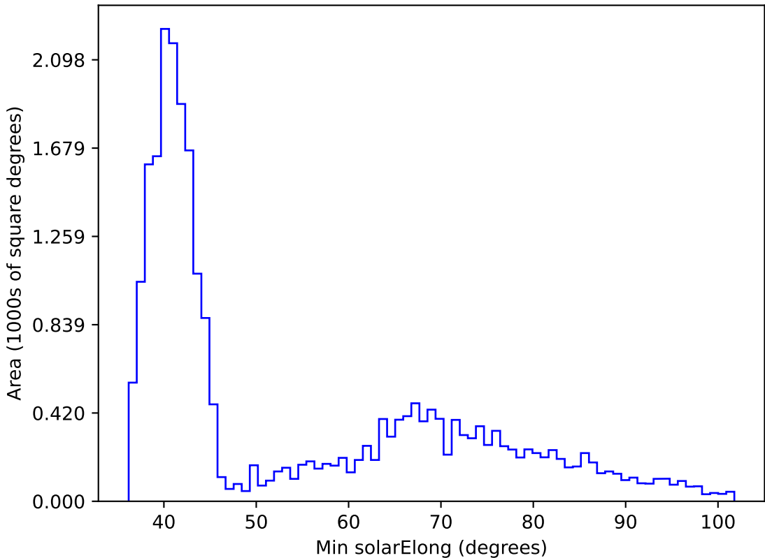
too_elab_r8_d2_gz_v3.4_10yrs All sky z band: Min solarElong
