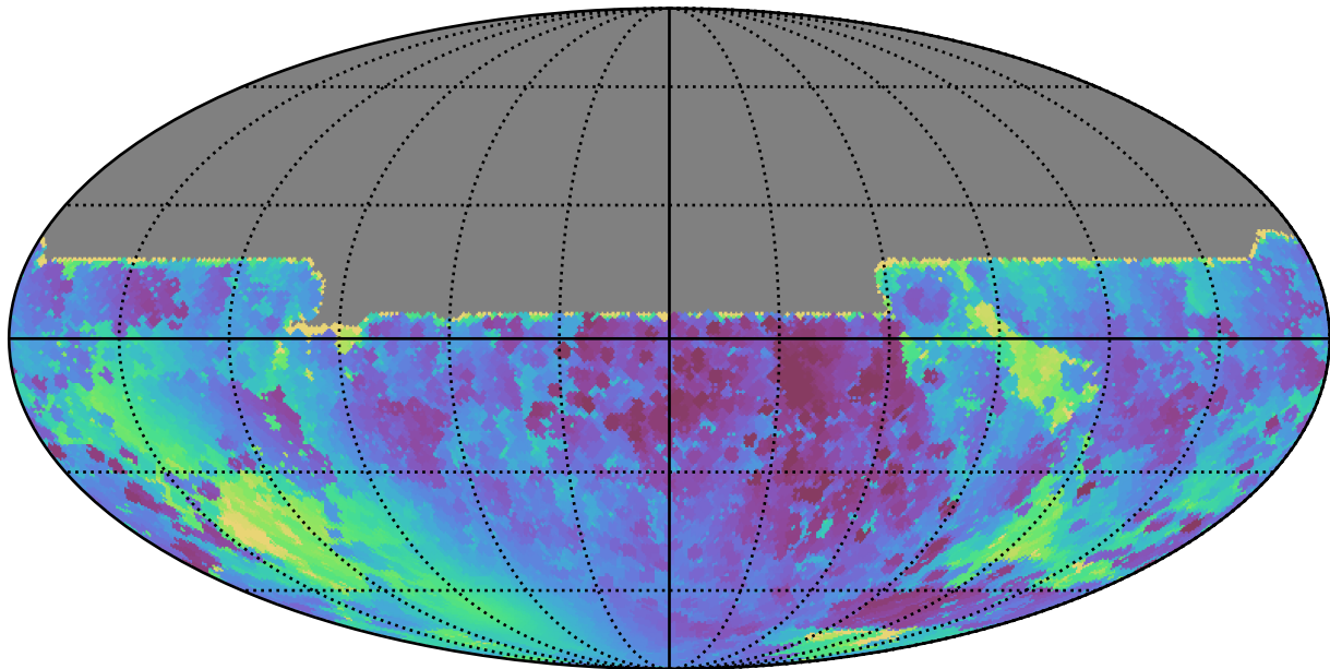
too_elab_r8_d2_gz_v3.4_10yrs All sky y band: Min solarElong
