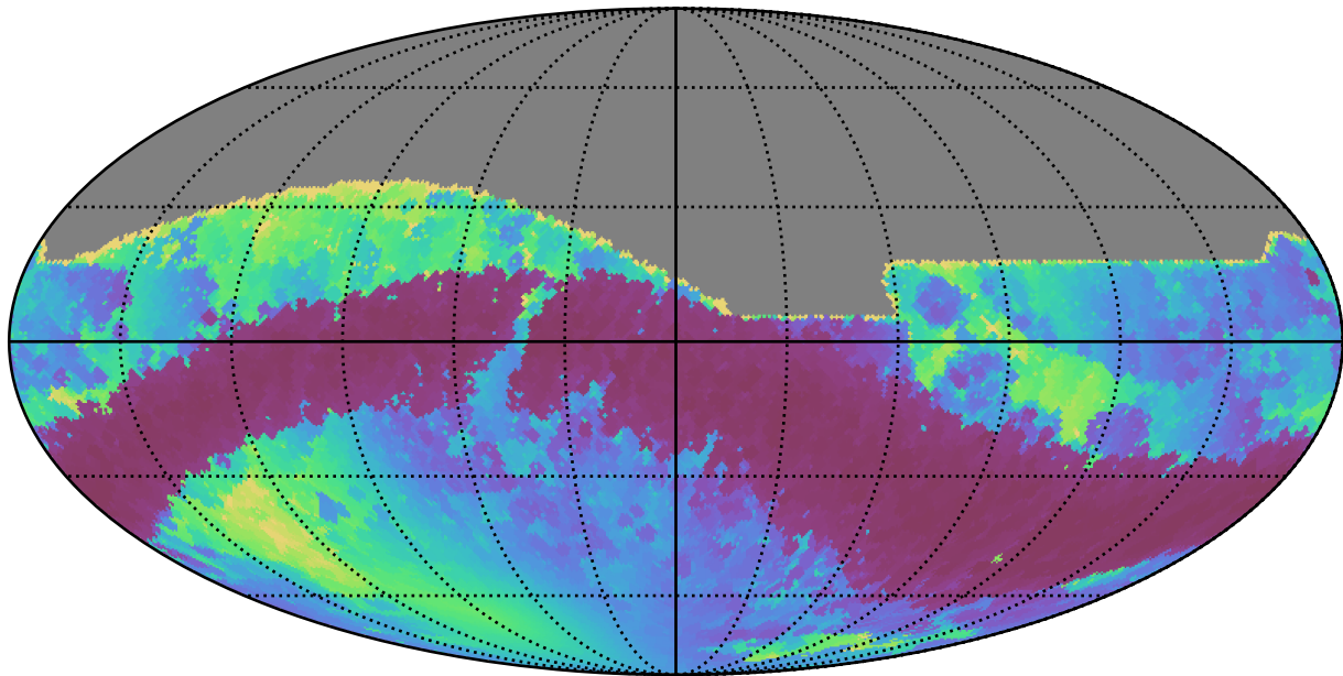
too_elab_r8_d2_gz_v3.4_10yrs All sky r band: Min solarElong
