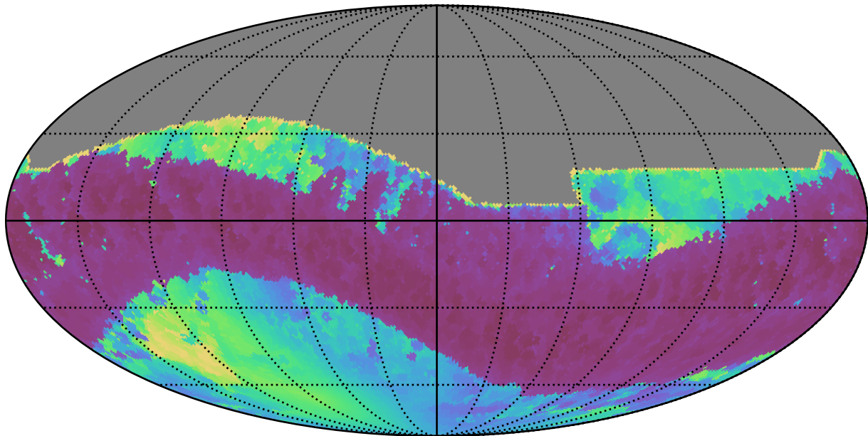
too_elab_r8_d2_gz_v3.4_10yrs All sky i band: Min solarElong
