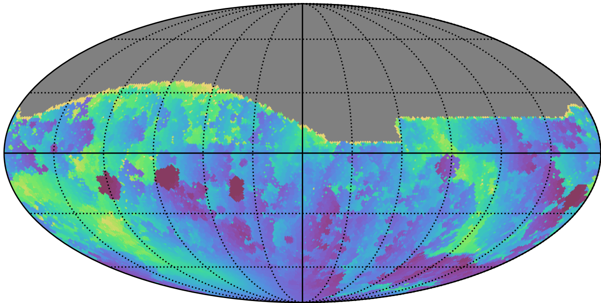
too_elab_r8_d2_gz_v3.4_10yrs All sky g band: Min solarElong
