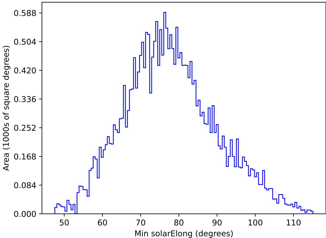
too_elab_r8_d2_gz_v3.4_10yrs All sky g band: Min solarElong
