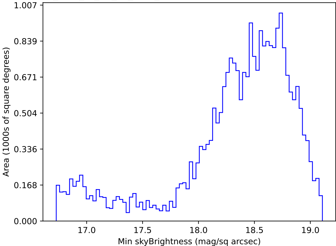
too_elab_r8_d2_gz_v3.4_10yrs Yr 1 z band: Min skyBrightness
