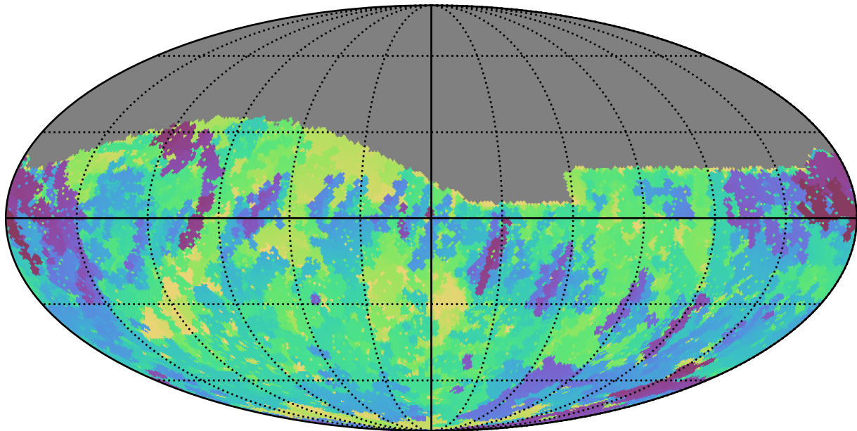
too_elab_r8_d2_gz_v3.4_10yrs Yr 1 r band: Min skyBrightness
