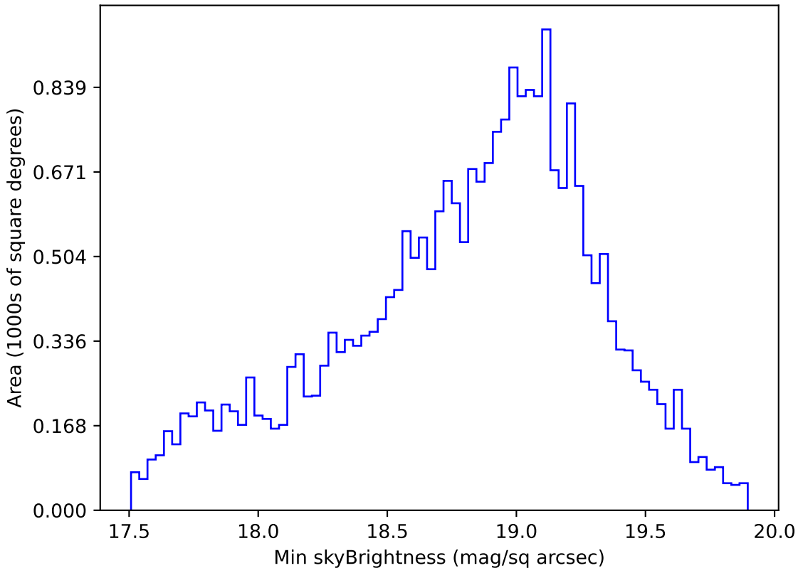
too_elab_r8_d2_gz_v3.4_10yrs Yr 1 i band: Min skyBrightness
