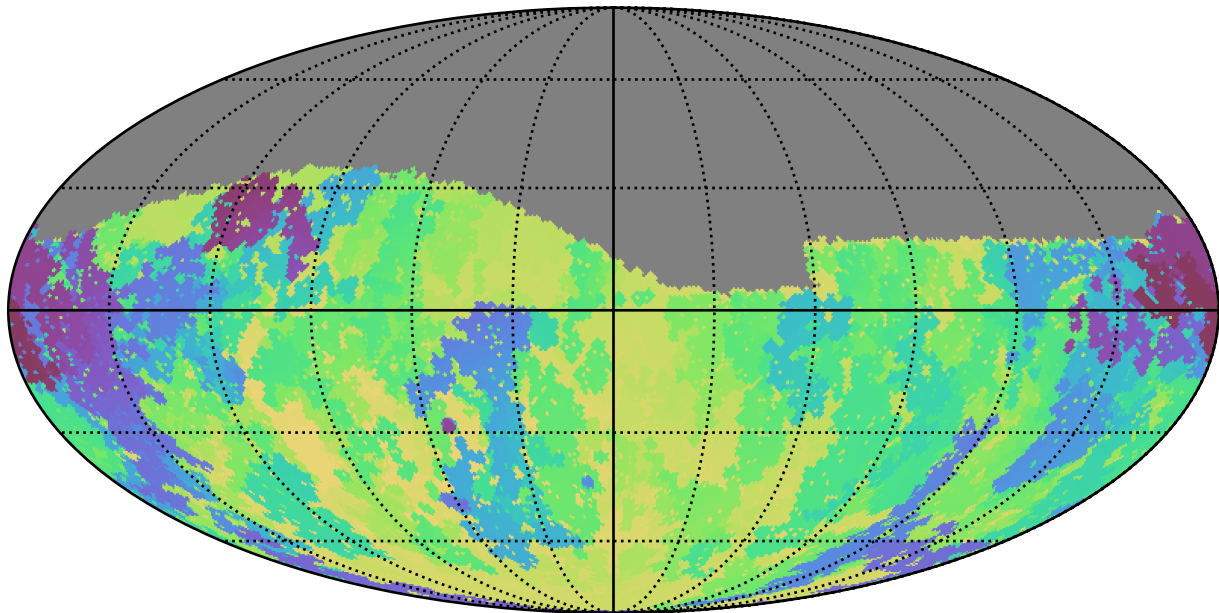
too_elab_r8_d2_gz_v3.4_10yrs Yr 1 g band: Min skyBrightness
