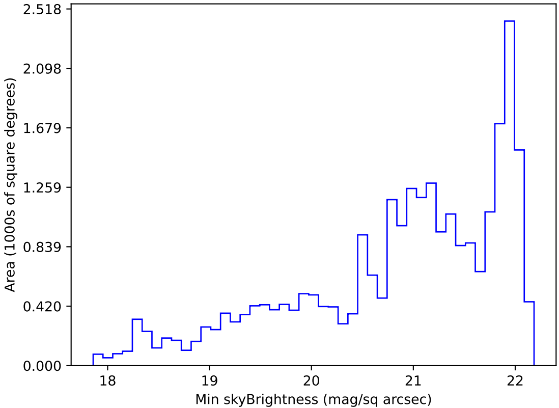
too_elab_r8_d2_gz_v3.4_10yrs Yr 1 g band: Min skyBrightness
