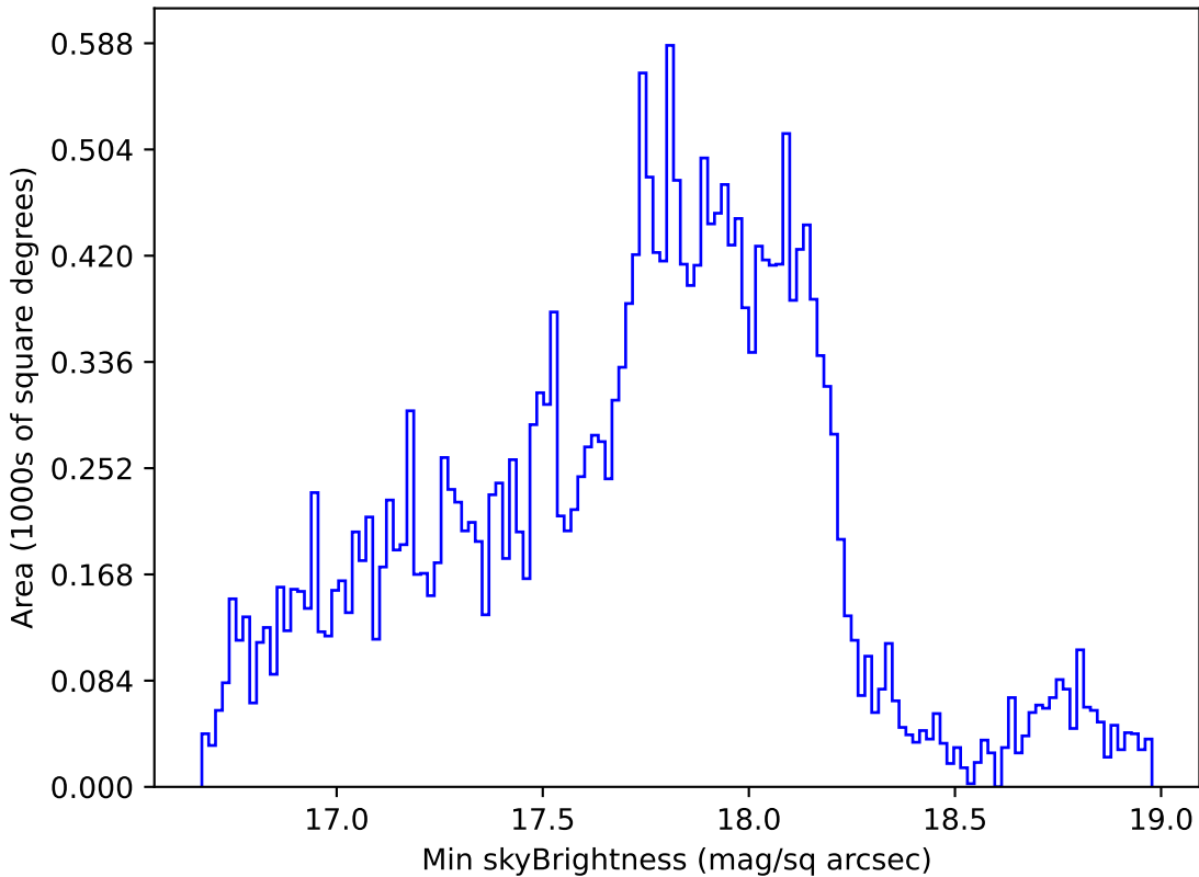
too_elab_r8_d2_gz_v3.4_10yrs Yr 1 all bands: Min skyBrightness
