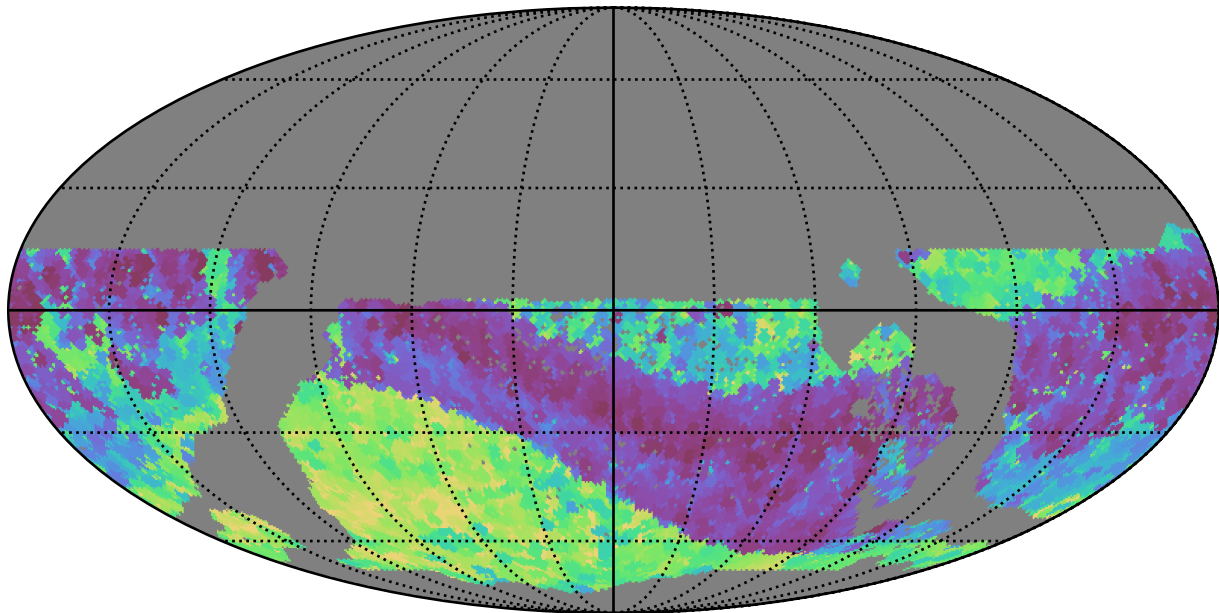
too_elab_r8_d2_gz_v3.4_10yrs WFD z band: Min skyBrightness
