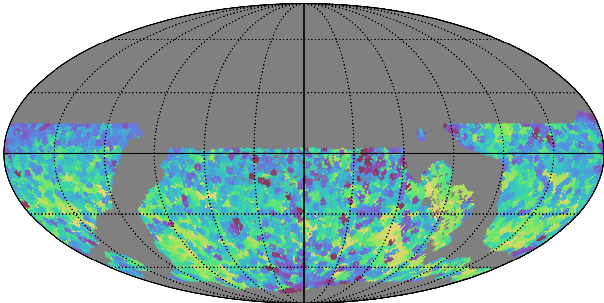
too_elab_r8_d2_gz_v3.4_10yrs WFD y band: Min skyBrightness
