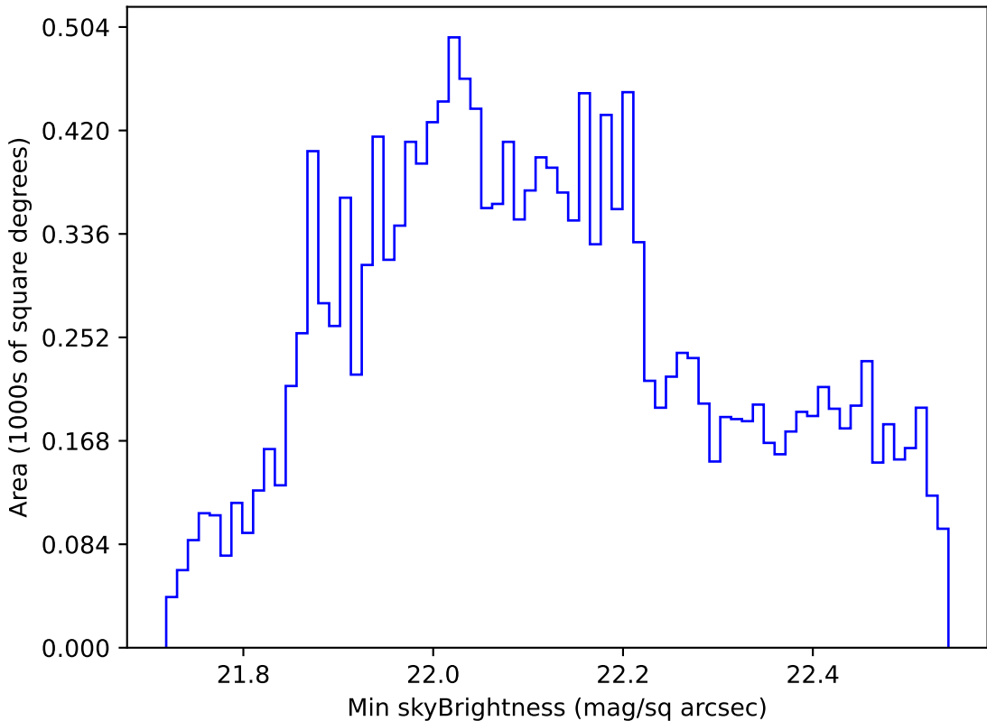
too_elab_r8_d2_gz_v3.4_10yrs WFD u band: Min skyBrightness
