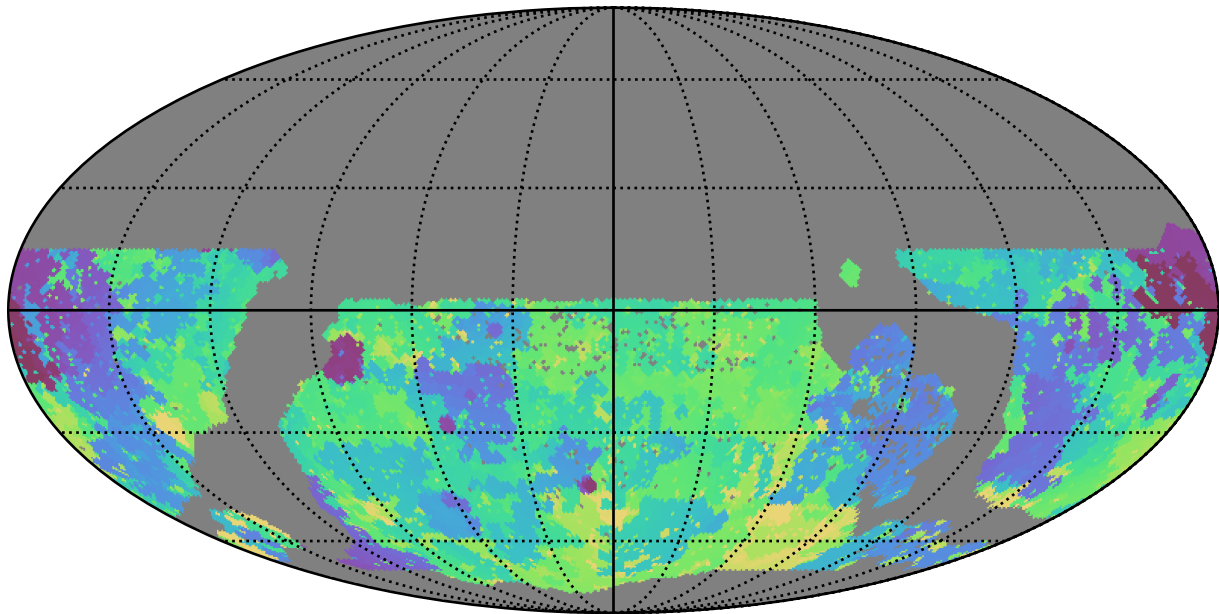
too_elab_r8_d2_gz_v3.4_10yrs WFD g band: Min skyBrightness
