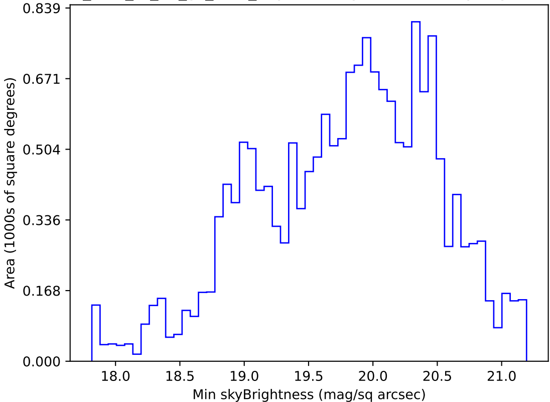
too_elab_r8_d2_gz_v3.4_10yrs WFD g band: Min skyBrightness
