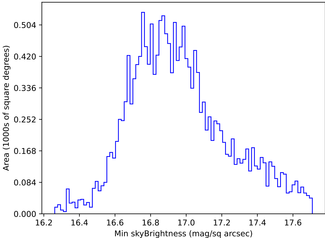
too_elab_r8_d2_gz_v3.4_10yrs WFD all bands: Min skyBrightness
