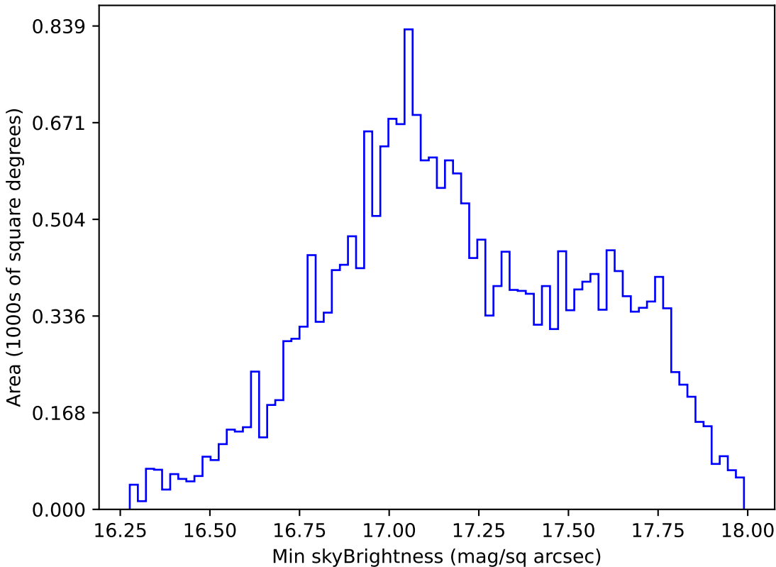
too_elab_r8_d2_gz_v3.4_10yrs All sky y band: Min skyBrightness
