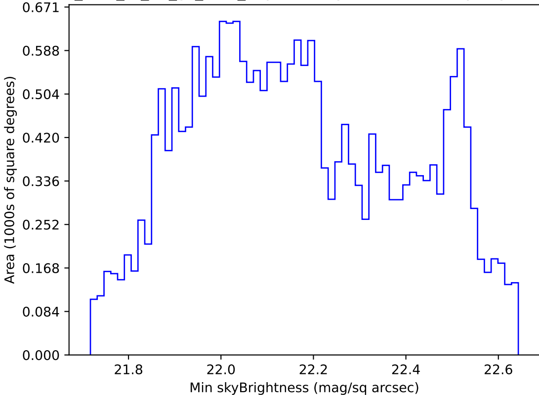
too_elab_r8_d2_gz_v3.4_10yrs All sky u band: Min skyBrightness
