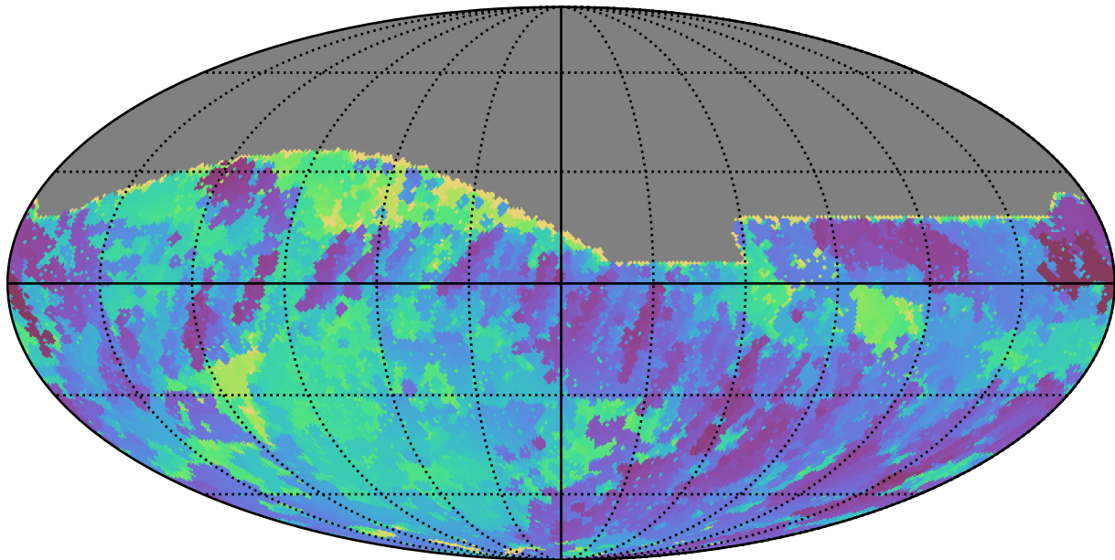
too_elab_r8_d2_gz_v3.4_10yrs All sky r band: Min skyBrightness
