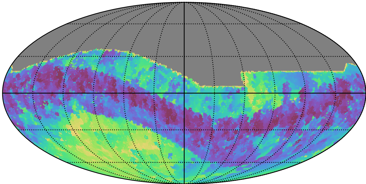
too_elab_r8_d2_gz_v3.4_10yrs All sky i band: Min skyBrightness
