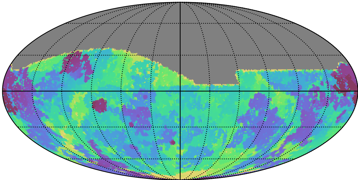
too_elab_r8_d2_gz_v3.4_10yrs All sky g band: Min skyBrightness
