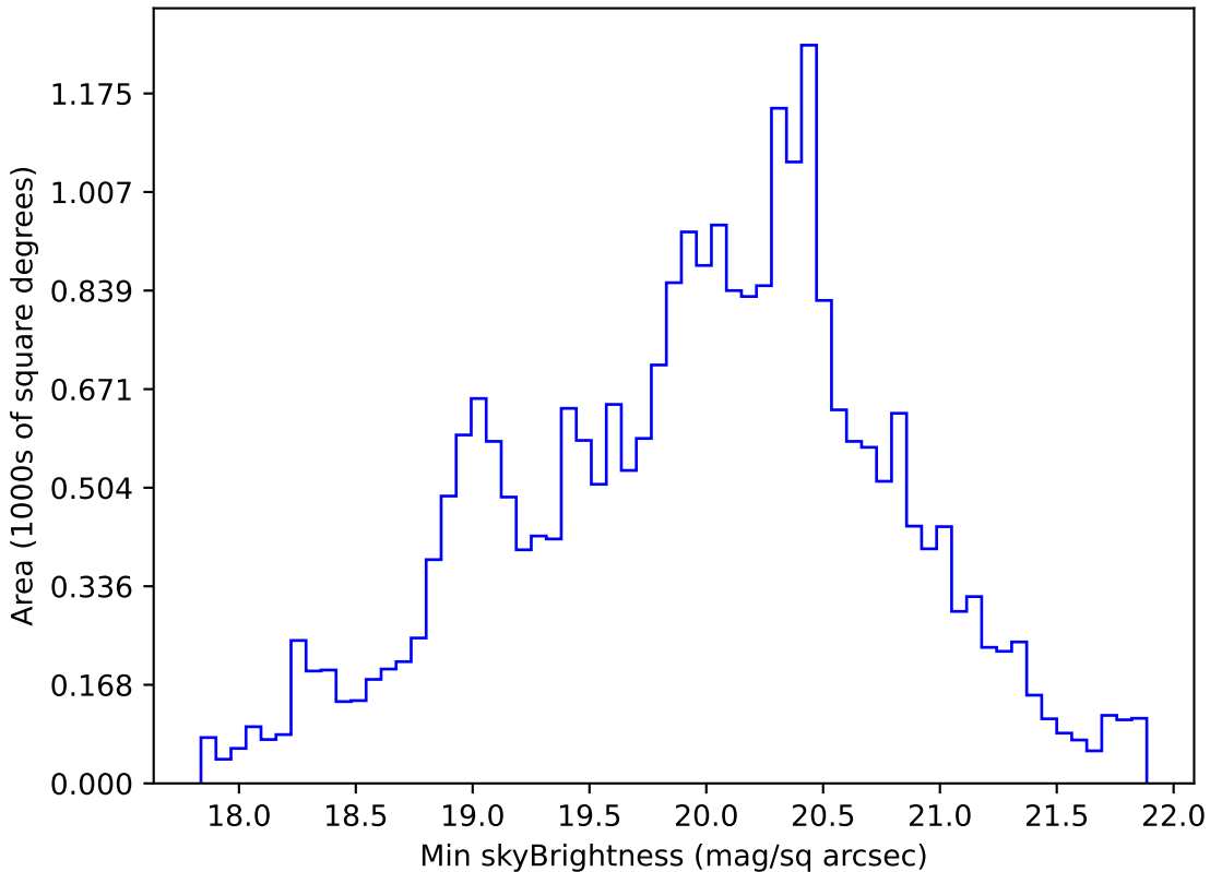
too_elab_r8_d2_gz_v3.4_10yrs All sky g band: Min skyBrightness
