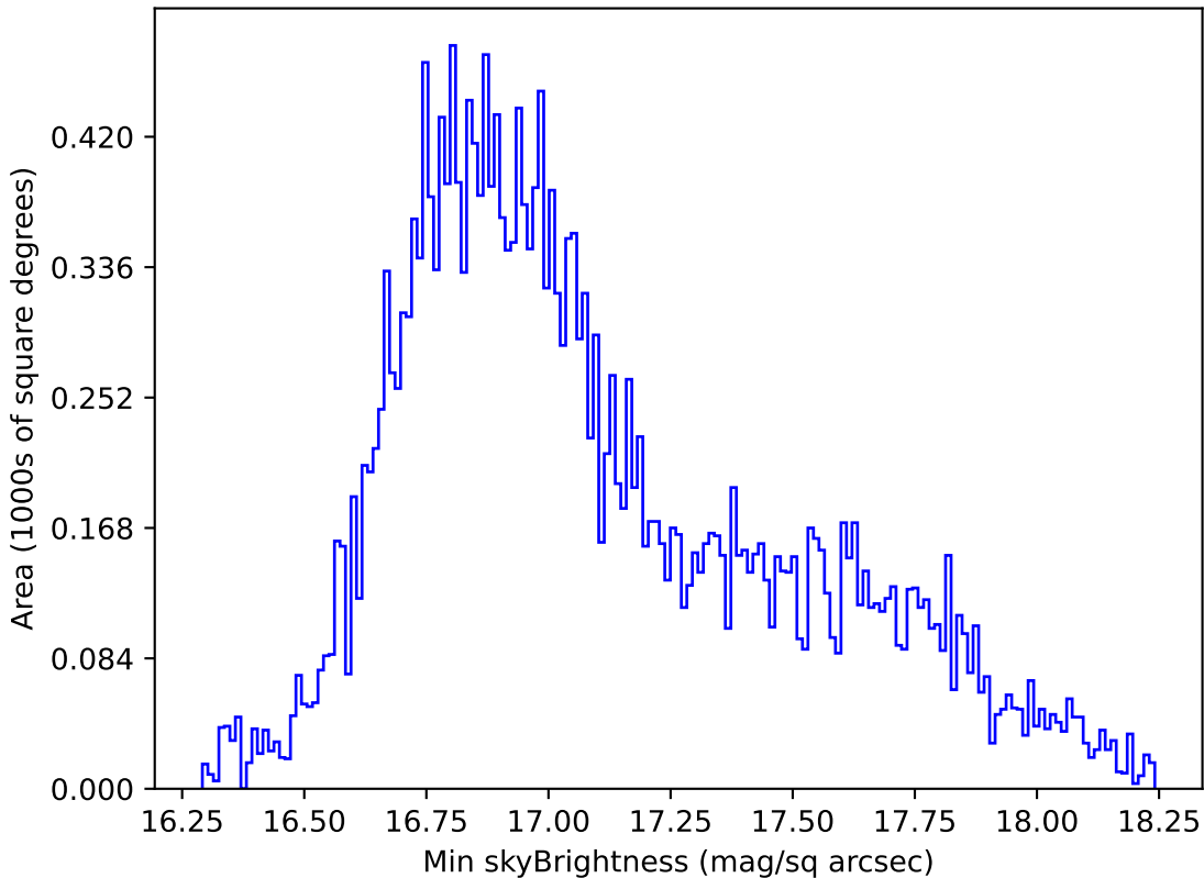
too_elab_r8_d2_gz_v3.4_10yrs All sky all bands: Min skyBrightness
