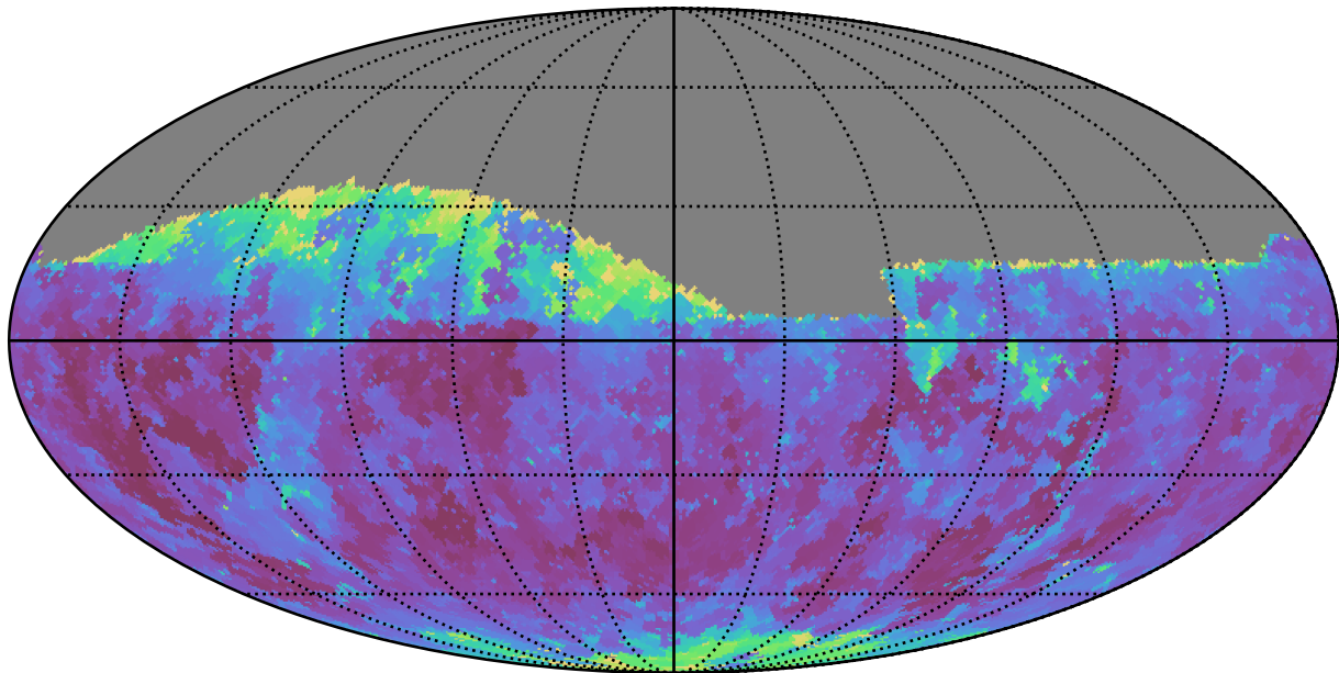
too_elab_r8_d2_gz_v3.4_10yrs Yr 1 z band: Min seeingGeom
