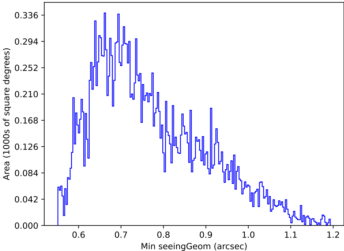
too_elab_r8_d2_gz_v3.4_10yrs Yr 1 u band: Min seeingGeom
