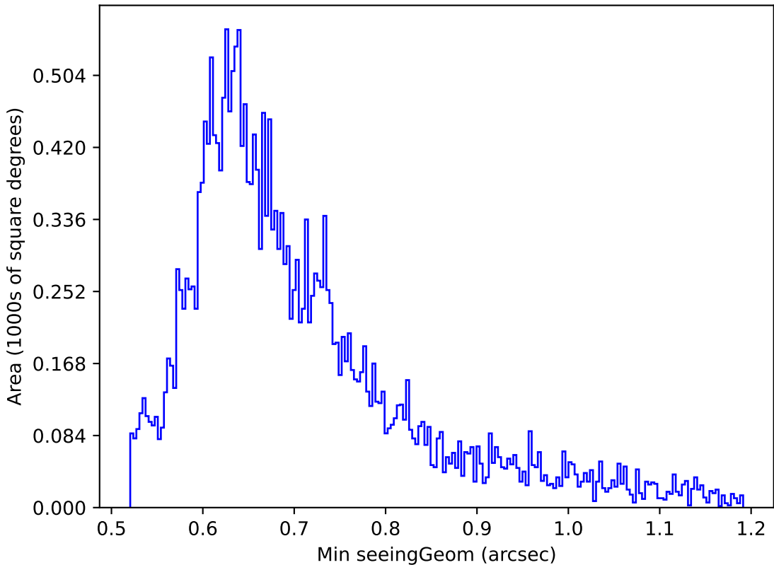
too_elab_r8_d2_gz_v3.4_10yrs Yr 1 g band: Min seeingGeom
