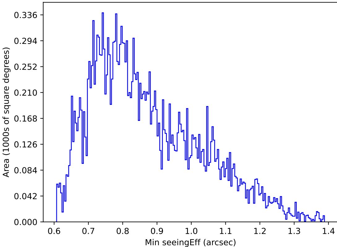
too_elab_r8_d2_gz_v3.4_10yrs Yr 1 u band: Min seeingEff
