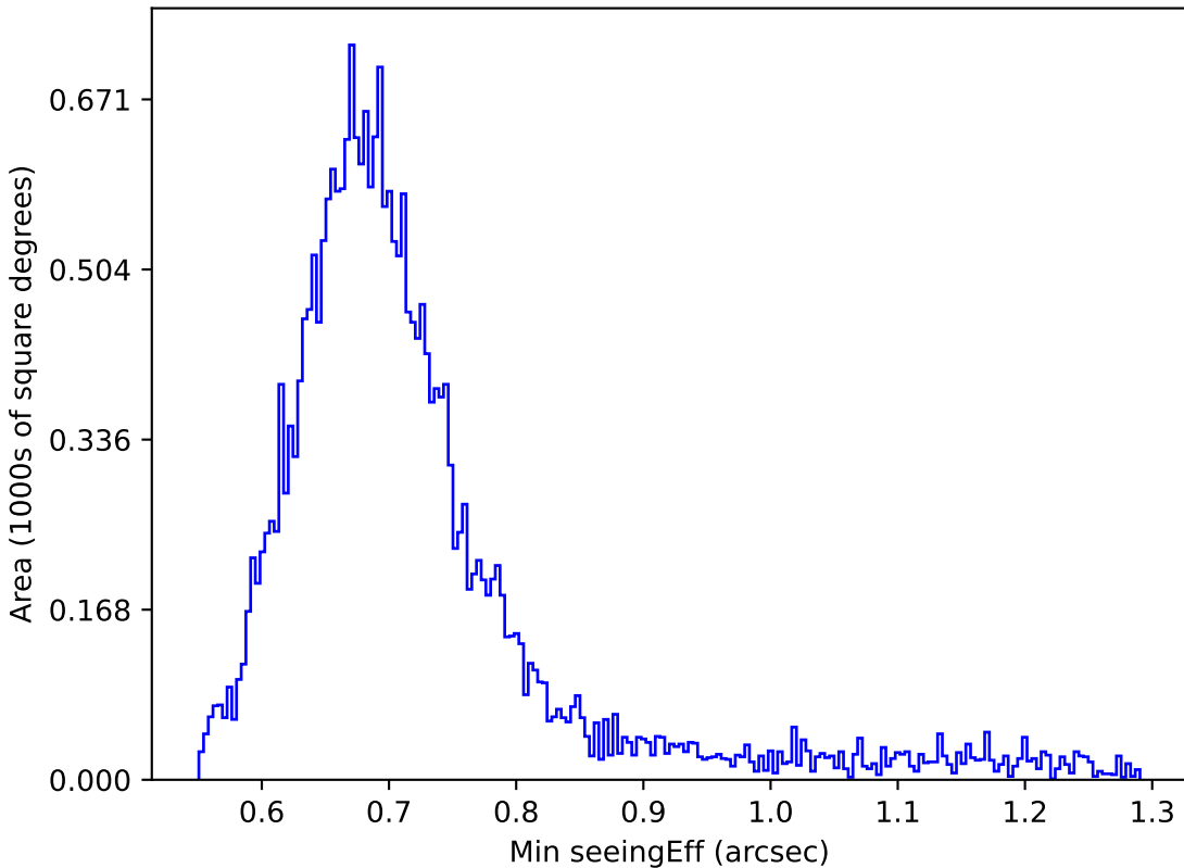
too_elab_r8_d2_gz_v3.4_10yrs Yr 1 r band: Min seeingEff
